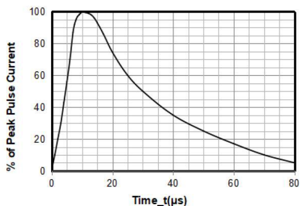
8 X 20 \mu\text{s} Pulse Waveform
