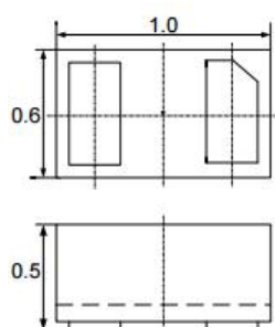
Package Dimensions
